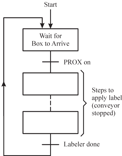
Figure 6.2. Chart of labeling station operation.
