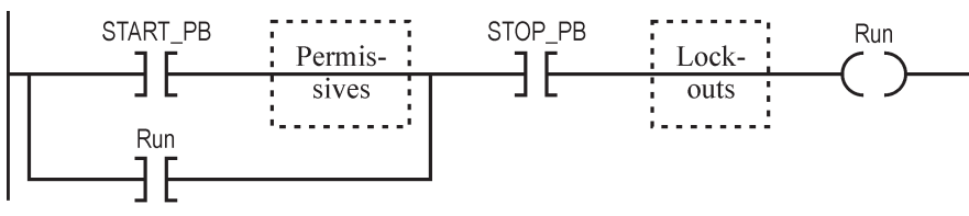
Figure 6.8. General start/stop/pause rung.
