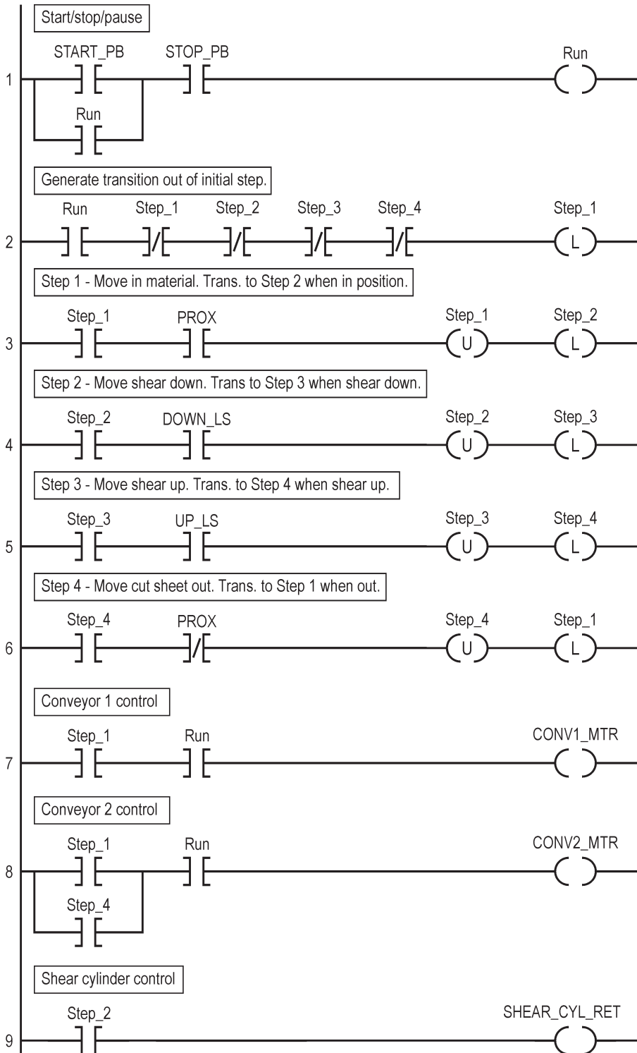
Figure 6.12. Ladder logic for metal shear.
