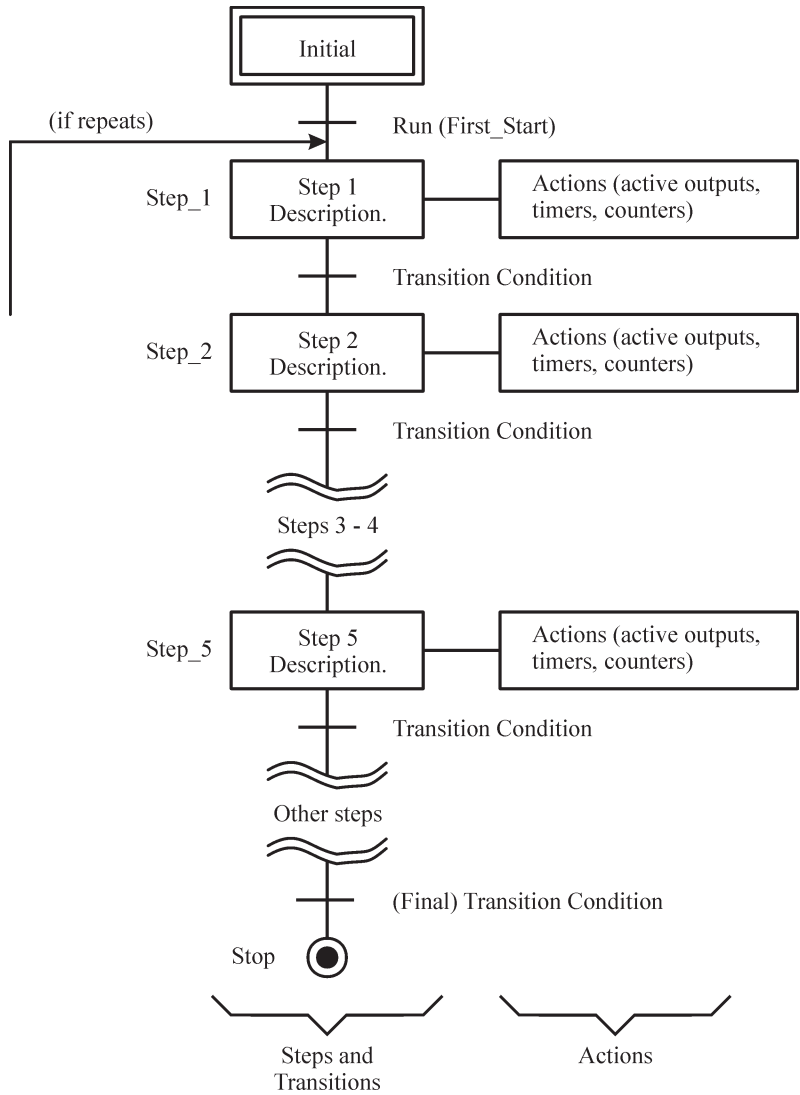
Figure 6.4. General function chart.
