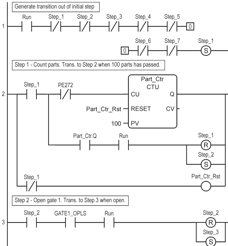
Figure 6.17. Micro800 ladder logic for tub loader. (continued)
