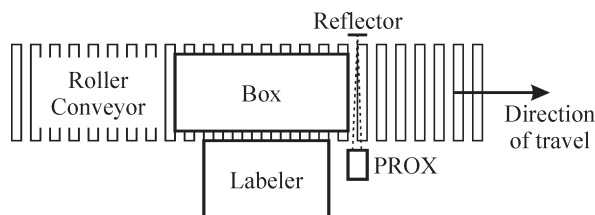
Figure 6.1. Labeling station.
