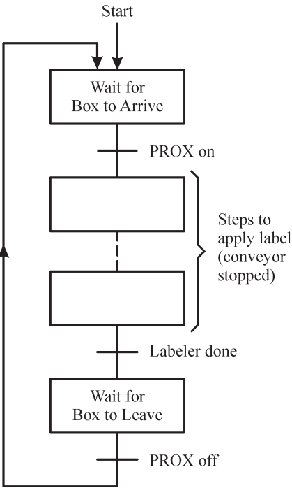
Figure 6.3. Corrected chart of labeling station operation.
