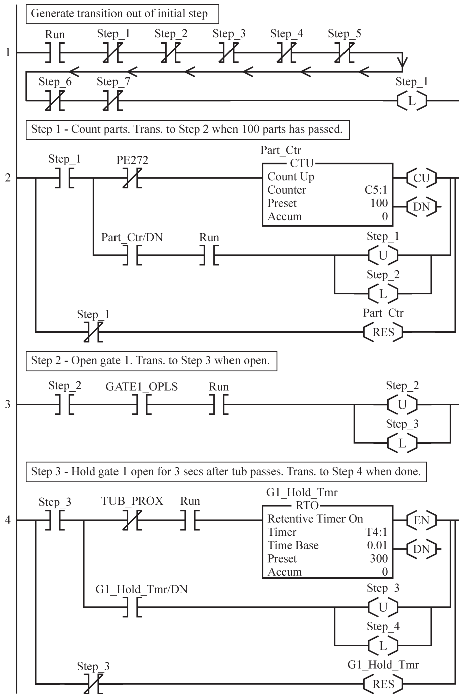
Figure 6.18. MicroLogix ladder logic for tub loader. (continued)
