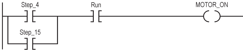
Figure 6.11. Example step action.
