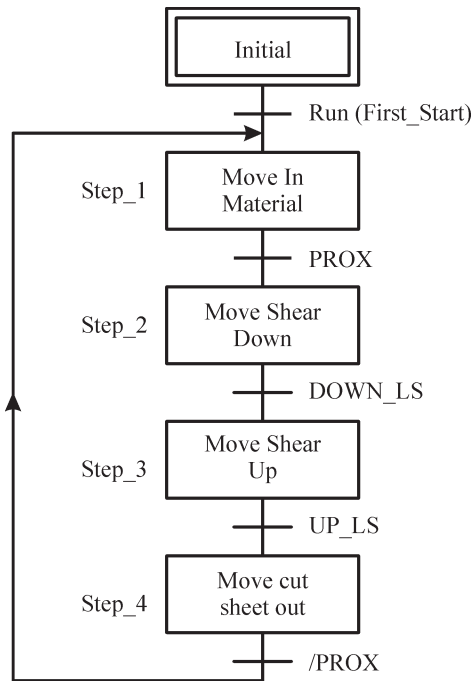
Figure 6.6. Steps and transitions for metal shear.
