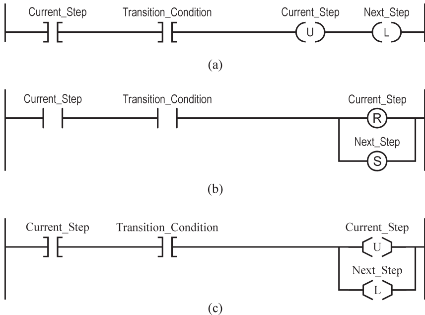
Figure 6.10. General transition between steps: (a) ControlLogix; (b) Micro800; (c) MicroLogix.
