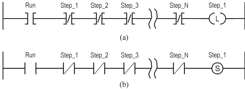
Figure 6.9. General first start rung: (a) ControlLogix and MicroLogix; (b) Micro800.
